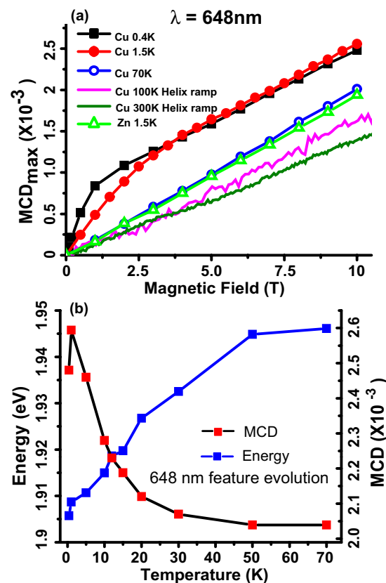
Figure 3. MCD signatures of spin exchange in Cu-OBPc thin films. (a) MCD ( \lambda = 648\text{ nm} ) evolution with increasing magnetic field in Cu-OBPc and Zn-OBPc at various temperatures ranging from 0.4 K to 300 K. For temperatures larger than 70 K MCD was measured in a continuous field sweep from 0 T to 25 T Split-Florida Helix magnet. (b) Evolution of the \lambda = 648\text{ nm} MCD with temperature for Cu-OBPc.
