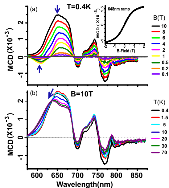
Figure 2. Magnetic field and temperature dependence of MCD in Cu-OBPc thin films. (a) MCD spectra of Cu-OBPc polycrystalline thin film recorded at T = 0.4\text{ K} and varying magnetic fields up to 10 T. Inset: MCD vs. B recorded at \lambda = 648\text{ nm} during a magnetic field ramp (b) MCD spectra from the same film recorded at B = 10\text{ T} and varying temperatures up to 70 K.
