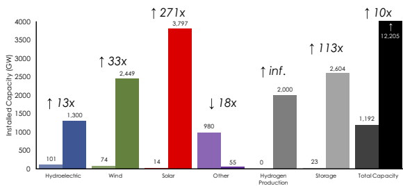
Fig. 2. Installed capacity values for 2015 (left column in each pair) and those used in the studies in refs. 11 and 12 (right column in each pair). These 100% wind, solar, and hydroelectric studies propose installing technologies at a scale equivalent to (or substantially greater than) the entire capacity of the existing electricity generation infrastructure. The other category includes coal, natural gas, and nuclear, all of which are removed by 2050.
