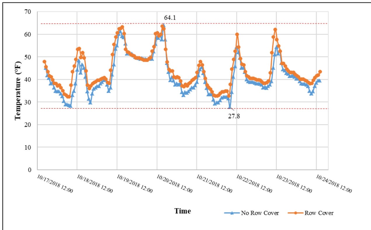
Figure 1. Average hourly temperatures at the base of the plants in row covered plots and uncovered plots.
