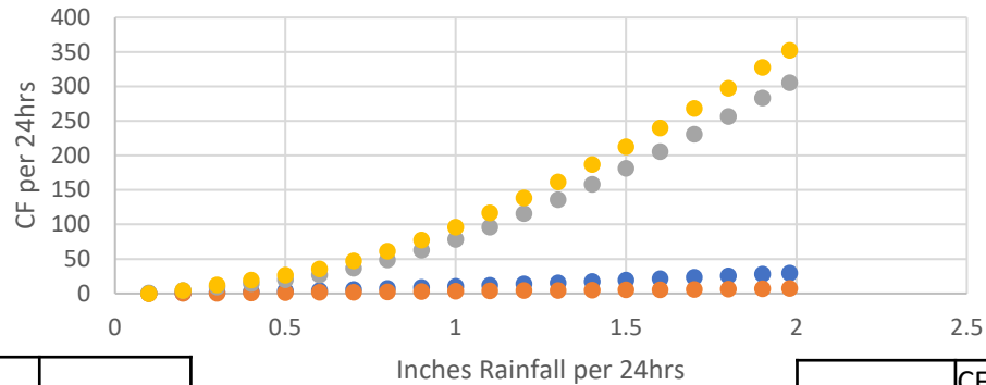
Fairview 100% Modeled Rainfall to outflow
