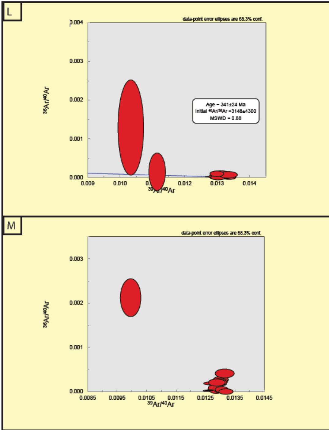
Appendix 2: Inverse Isochron plots for each of the samples. A: Sample 18CD08B Biotite. B: Sample 18CD08B Hornblende. C: Sample 18CD08D Biotite. D: Sample 18CD08D White Mica. E: Sample 18CD08E Biotite #1. F: Sample 18CD08E Biotite #2. G: Sample 18CD08E White Mica. H: Sample 18CD10A Biotite. I: Sample 18CD10A White Mica. J: Sample 18CD10B Hornblende #1. K: Sample 18CD10B Hornblende#2. L: Sample 18CD10C Biotite. M: Sample 18CD10C White Mica.
