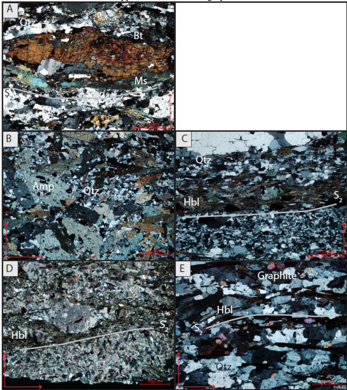
Appendix 4: Photomicrographs of the samples not subjected to ^{40}\text{Ar}/^{39}\text{Ar} geochronology. Qtz = Quartz, Bt = Biotite, Ms = Muscovite, S 2 = Foliation, Amp = Amphibole, Hbl = Hornblende. A: Sample 18CD08C containing quartz biotite and muscovite. There is foliation defined by layering of mica and quartz. B: Sample 18CD09A contains quartz and amphibole. There is no foliation in this sample. C: Sample 18CD09B containing quartz and hornblende. The foliation is defined by a preferred orientation in the hornblende. D: Sample 18CD09C contains quartz and hornblende. The foliation is defined by compositional layering. E: Sample 18CD10D contains quartz, hornblende and graphite. The foliation is defined by orientation of hornblende.
