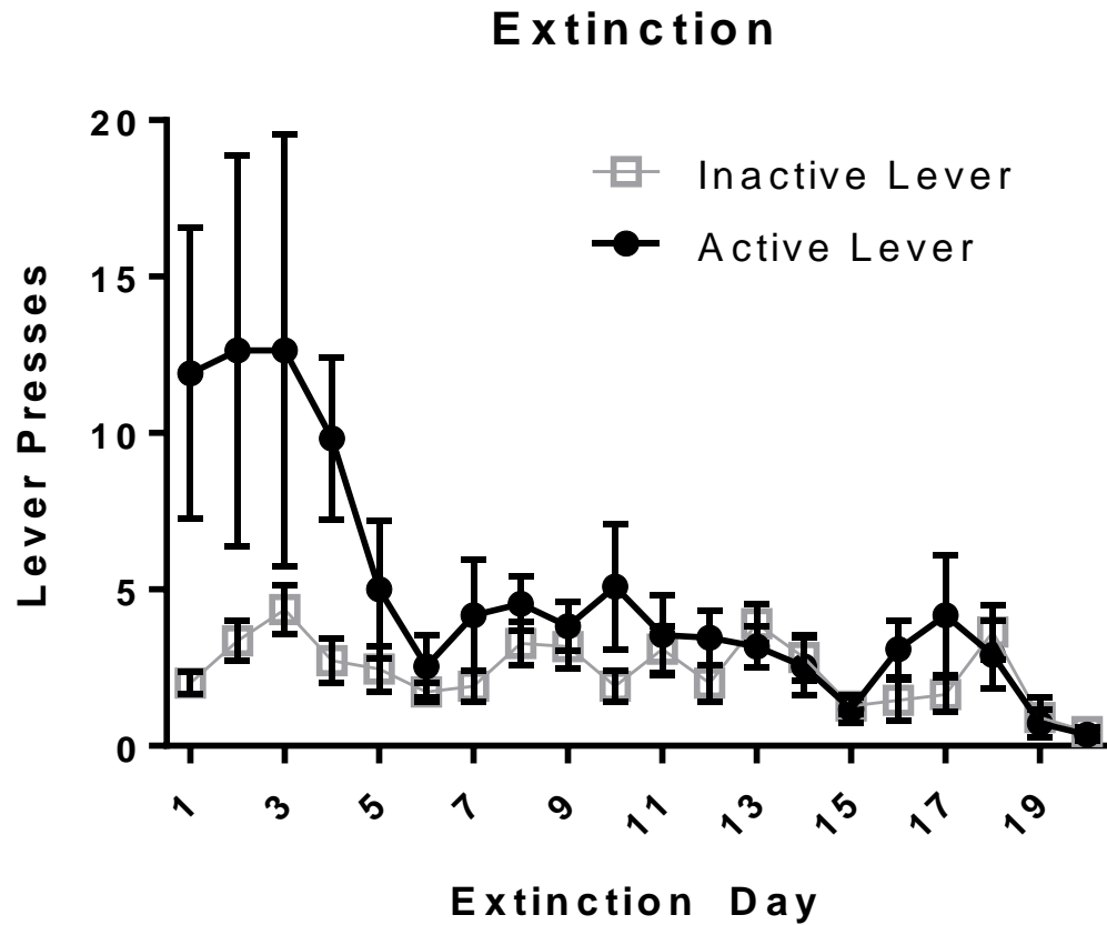
Figure 8: Extinction Training during Experiment 2.
