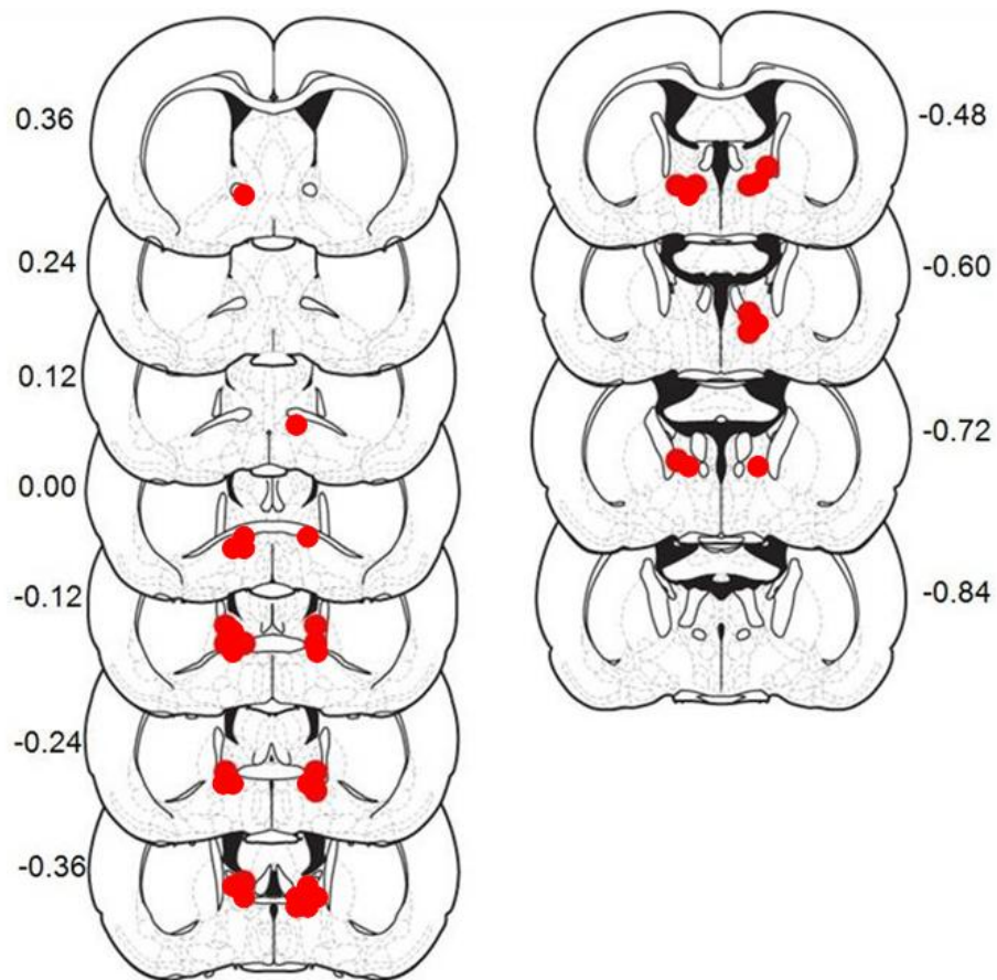
Figure 6: BNST Cannula Placements. Cannula placements for Experiment 2 are depicted above such that enclosed red circles represent a 1 mm extension beyond the tip of the cannula. Rats were included in analysis if their placement resided within a portion of the BNST.
