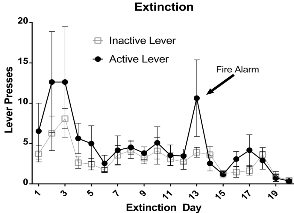
Figure 4: Extinction Training during Experiment 1. Extinction sessions occurred during the 20 days after self-administration training. Significant increases in responding on the first three days of extinction indicate awareness by the animals that the drug is no longer being delivered. On extinction day 13, a 30 min fire alarm interrupted extinction training, creating a stress-induced reinstatement-like response strictly on the active lever (previously associated with cocaine delivery).
