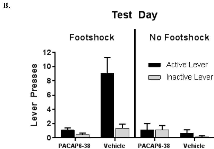
Figure 9: Intra-BNST PACAP6-38 attenuates stress-induced reinstatement when paired with intermittent, unpredictable footshock. A. Intra-BNST PACAP antagonist significantly attenuated stress-induced reinstatement when paired with a footshock when compared with the last day of extinction. Only animals who received intra-BNST vehicle treatment paired with a footshock demonstrated increased reinstatement to drug-seeking behaviors on the lever previously associated with cocaine delivery. B. Test for reinstatement by intermittent, unpredictable footshock.
