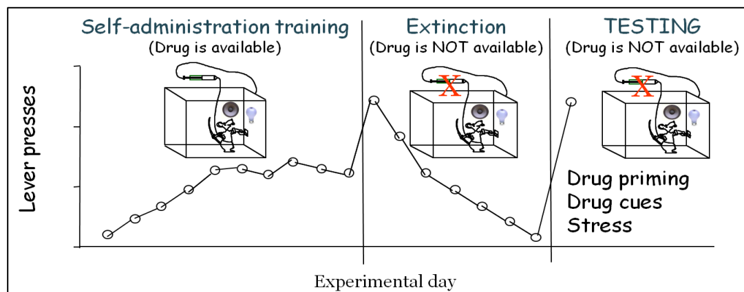
Figure 1. The Reinstatement Model of drug relapse. Representative self-administration paradigm, modified from a talk given by Yavin Shaham, PhD at the Neurobiology of Relapse Section, Behavioral Neuroscience Branch IRP/NIDA/NIH/DHHS, Baltimore. During acquisition, or self-administration training, animals are allowed to lever press for cocaine delivery for 10 days. During this period, lever press responses increase as animals continually seek the drug. Immediately following acquisition of drug-seeking, the behavior is extinguished in the Extinction phase. Here, lever press behavior is NOT followed by a drug stimulus and animals learn, over a 20-day extinction period, that lever presses no longer produce a drug reward. Finally, test day occurs one day following the termination of extinction. Reinstatement has been shown to occur with drug-priming, drug-cues and the presentation of a physical stressor.
