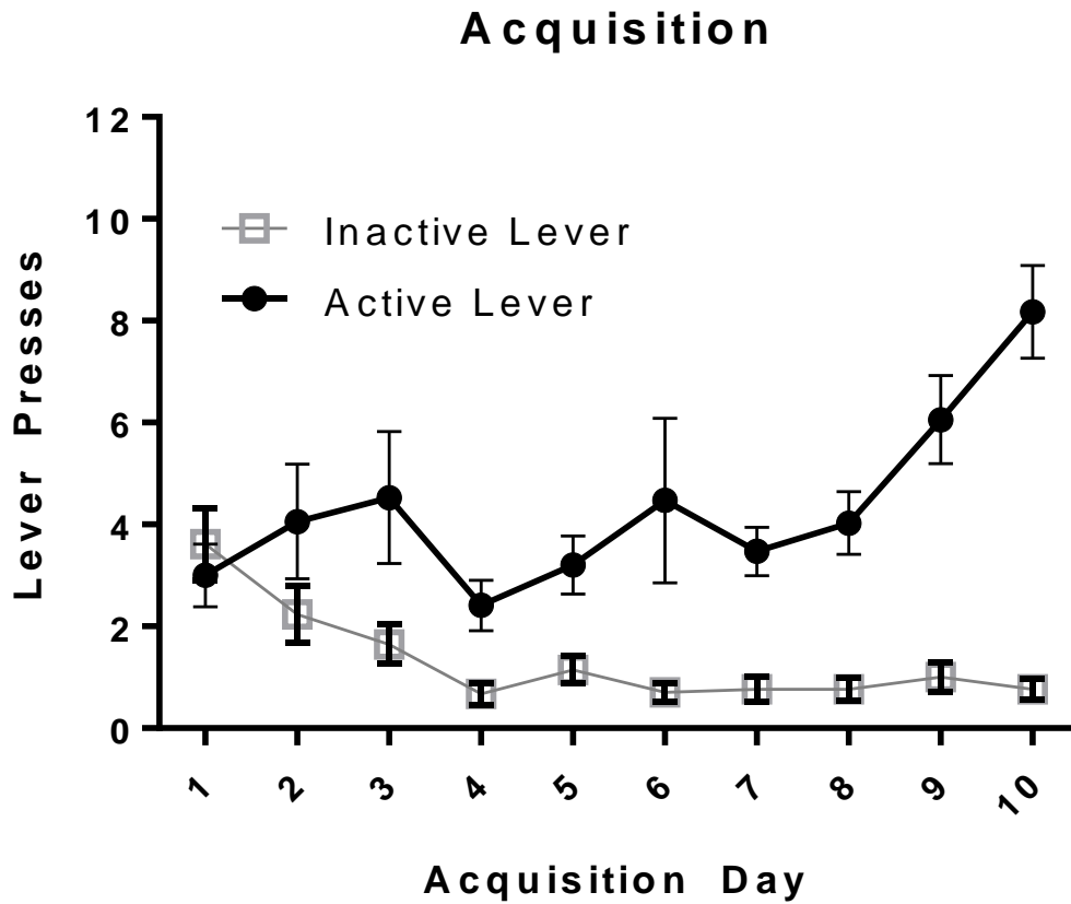
Figure 7: Self-Administration during Experiment 2.
