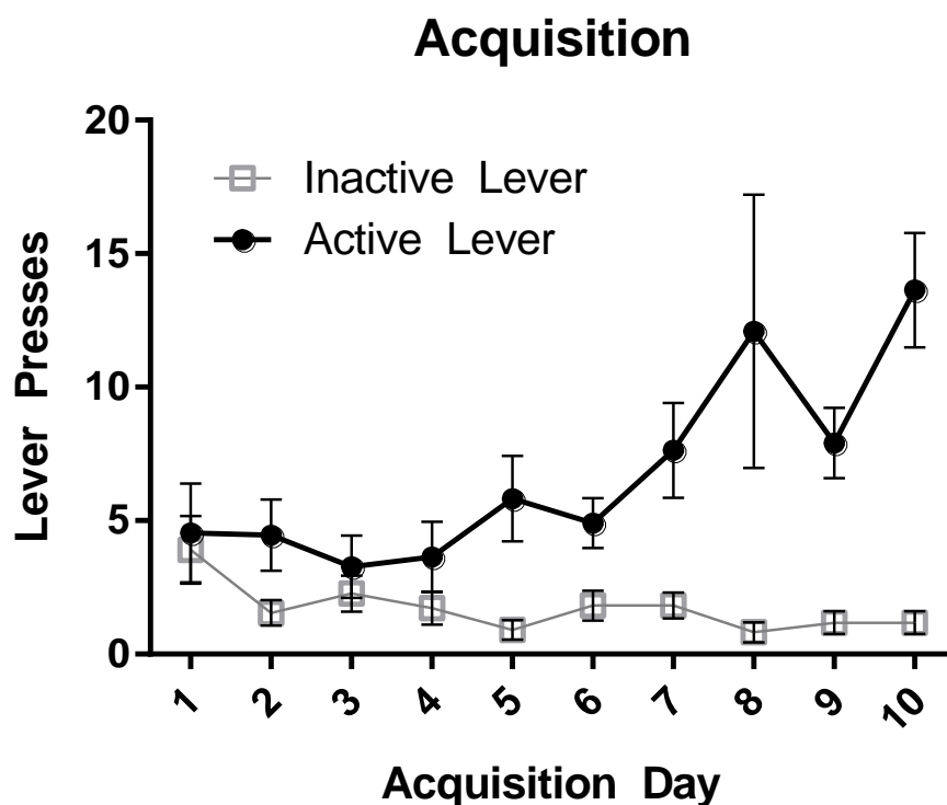
Figure 3: Self Administration training during Experiment 1.
