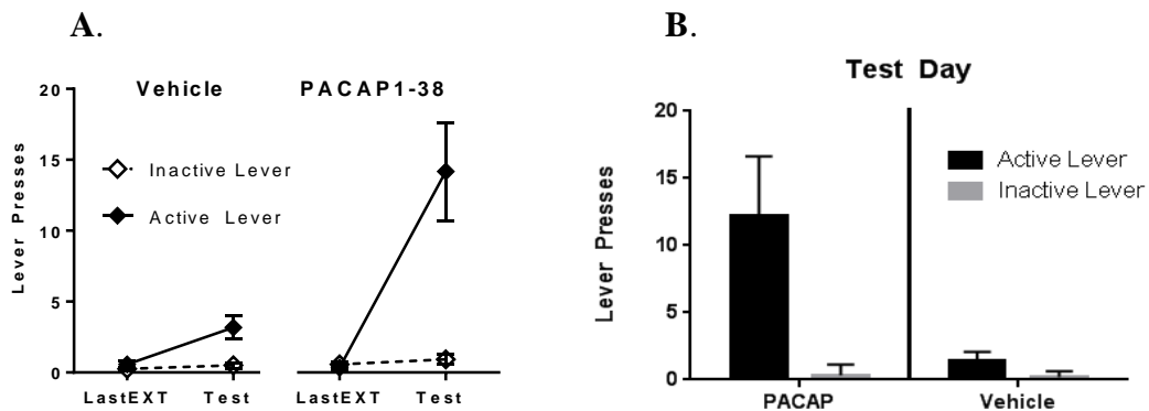
Figure 5: Intra-BNST PACAP38 causes reinstatement to drug-seeking. A,B. PACAP38 infusion causes significant reinstatement on the active lever (previously associated with cocaine delivery) during test for reinstatement compared to the last day of extinction (one day prior to test).
