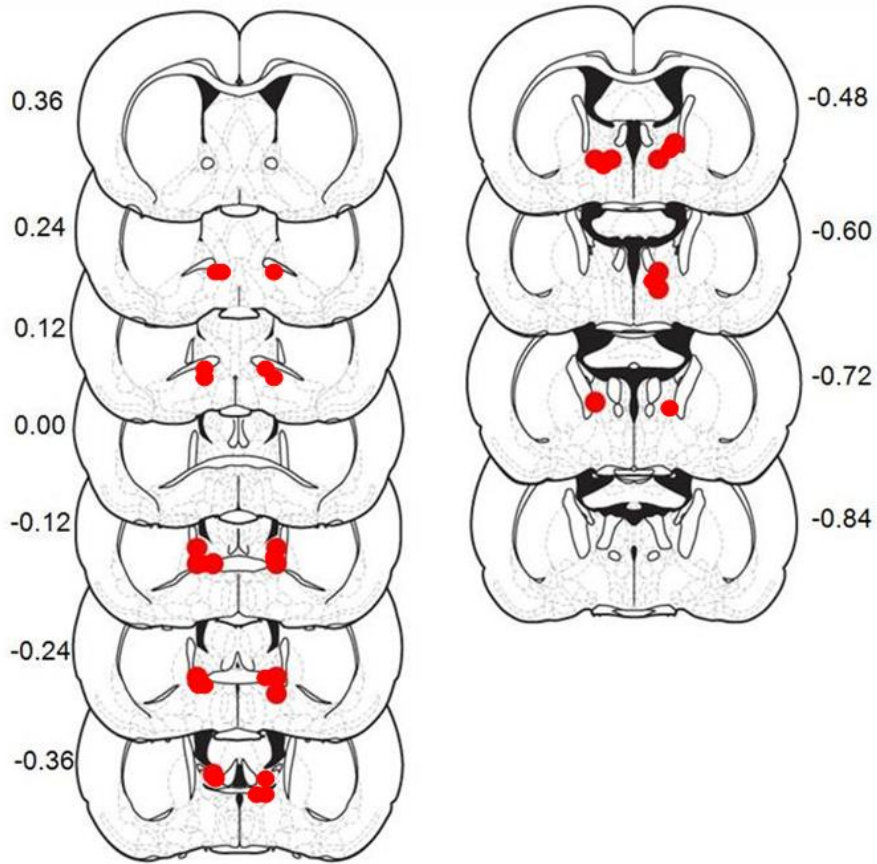
Figure 2: BNST Cannula Placements. Cannula placements for Experiment 1 are depicted above such that enclosed red dots represent a 1 mm extension beyond the tip of the cannula. Rats were included in the analysis if their placement resided within a portion of the BNST.
