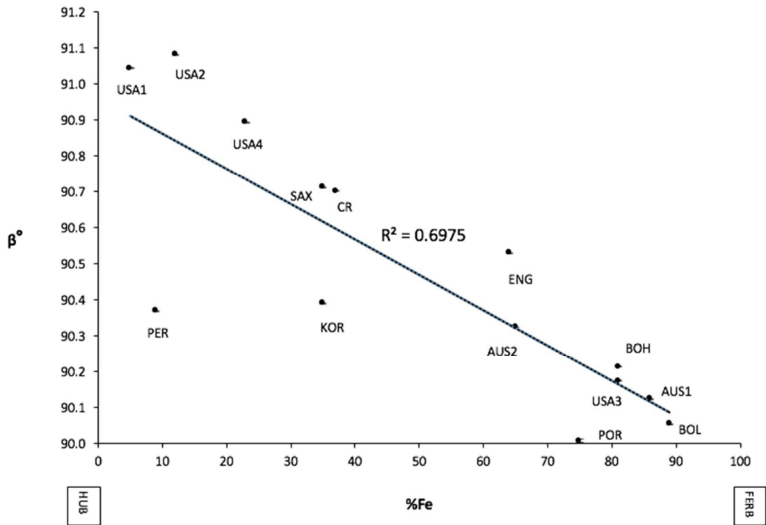
Figure 3-4. Composition versus Unit Cell Parameter \beta
