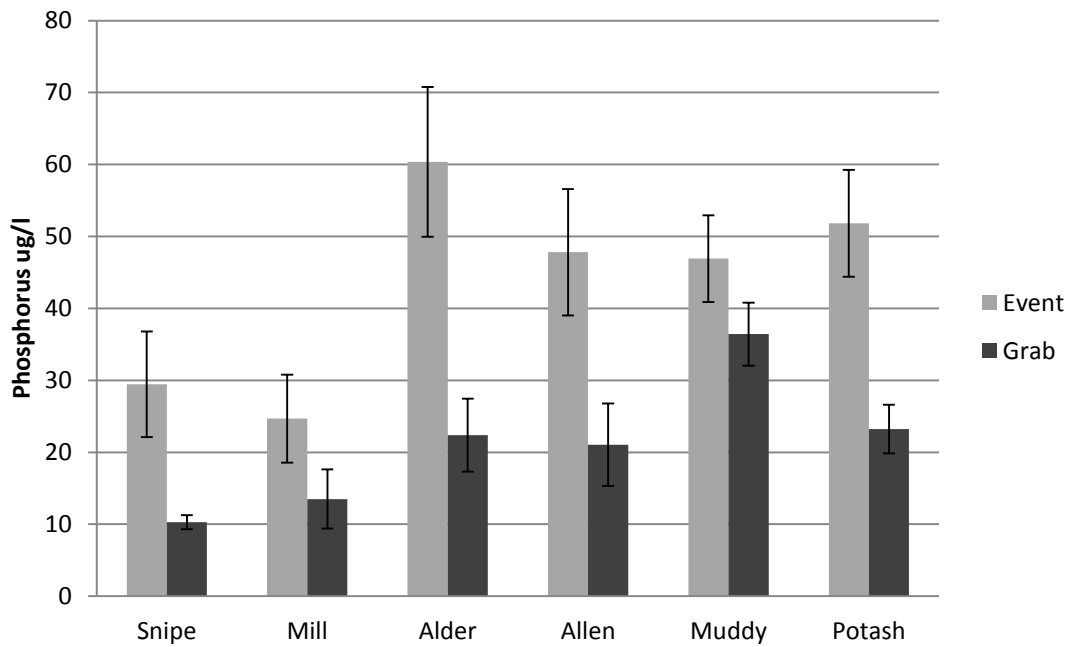
FIGURE 7. Mean total phosphorus concentrations for storm event and baseflow grab samples (error bars represent +/1 1 SE).
