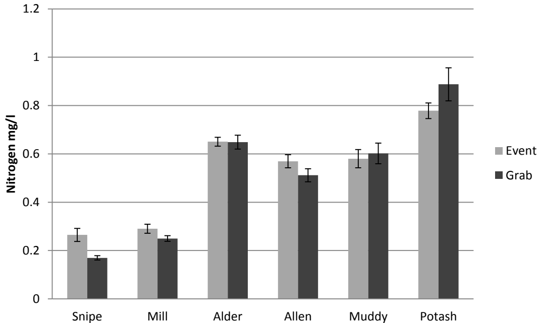
FIGURE 8. Mean total nitrogen concentrations for storm event and baseflow grab samples (error bars represent +/- 1 SE).
