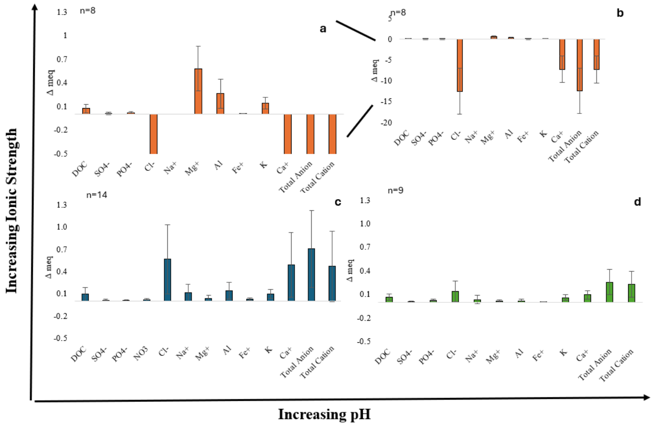
Figure 7: Change in solute composition (=outflow minus inflow) expressed as \Delta meq when treated with acid (a, see b for full scale), mixed (c), or recovery (d) inflow solution. Positive values indicate ion release from the soil core, negative values indicate ion retention in the soil core.
