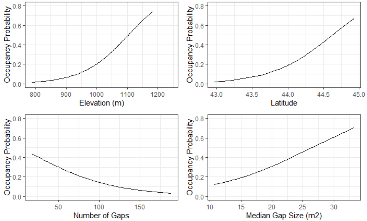
Figure 5: Predicted average occupancy probability of Bicknell's Thrush based on the detection covariates present in the final model. Occupancy was predicted using the logit-link function for the covariate of interest and the average value for all other covariates.
